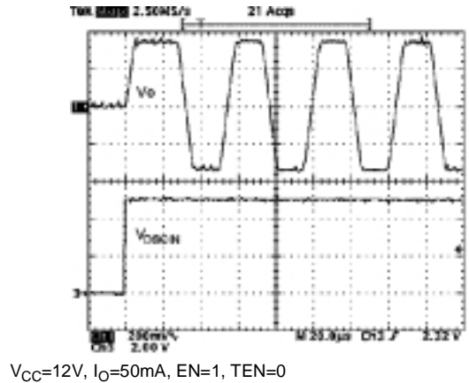
Figure 36: DSQIN Tone Enable Transient Response
