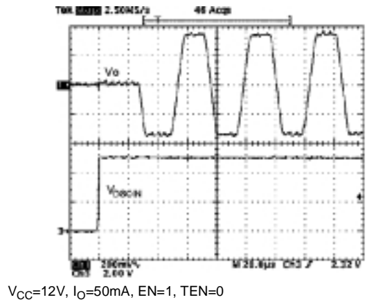
Figure 35: DSQIN Tone Enable Transient Response
