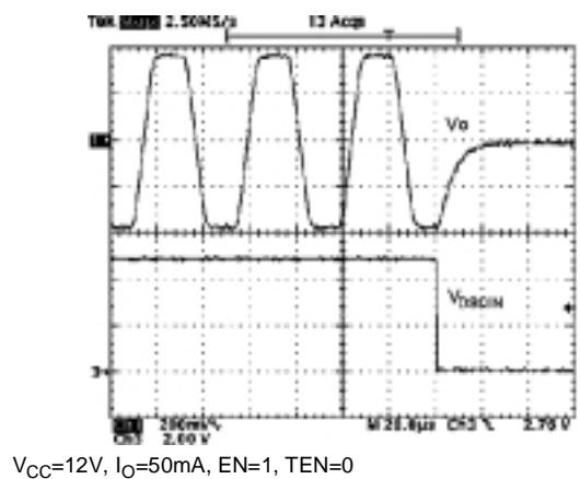
Figure 37: DSQIN Tone Disable Transient Response
