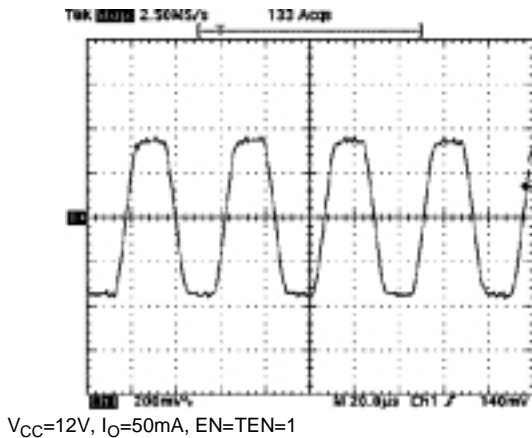
Figure 34: 22kHz Tone
